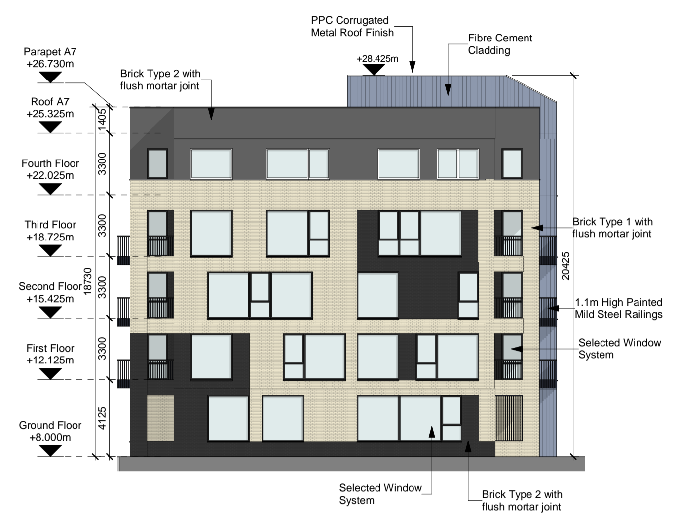
1 North Elevation 1 : 200
